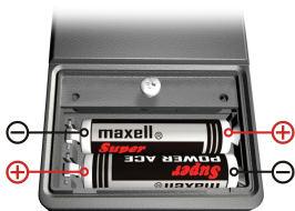
Pic. 4 Batteries installation scheme
